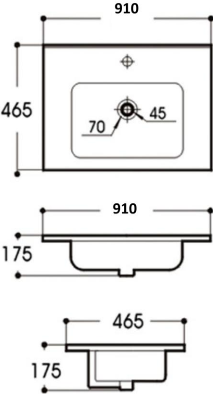
Technical Drawing / Dimensions / Detail View
